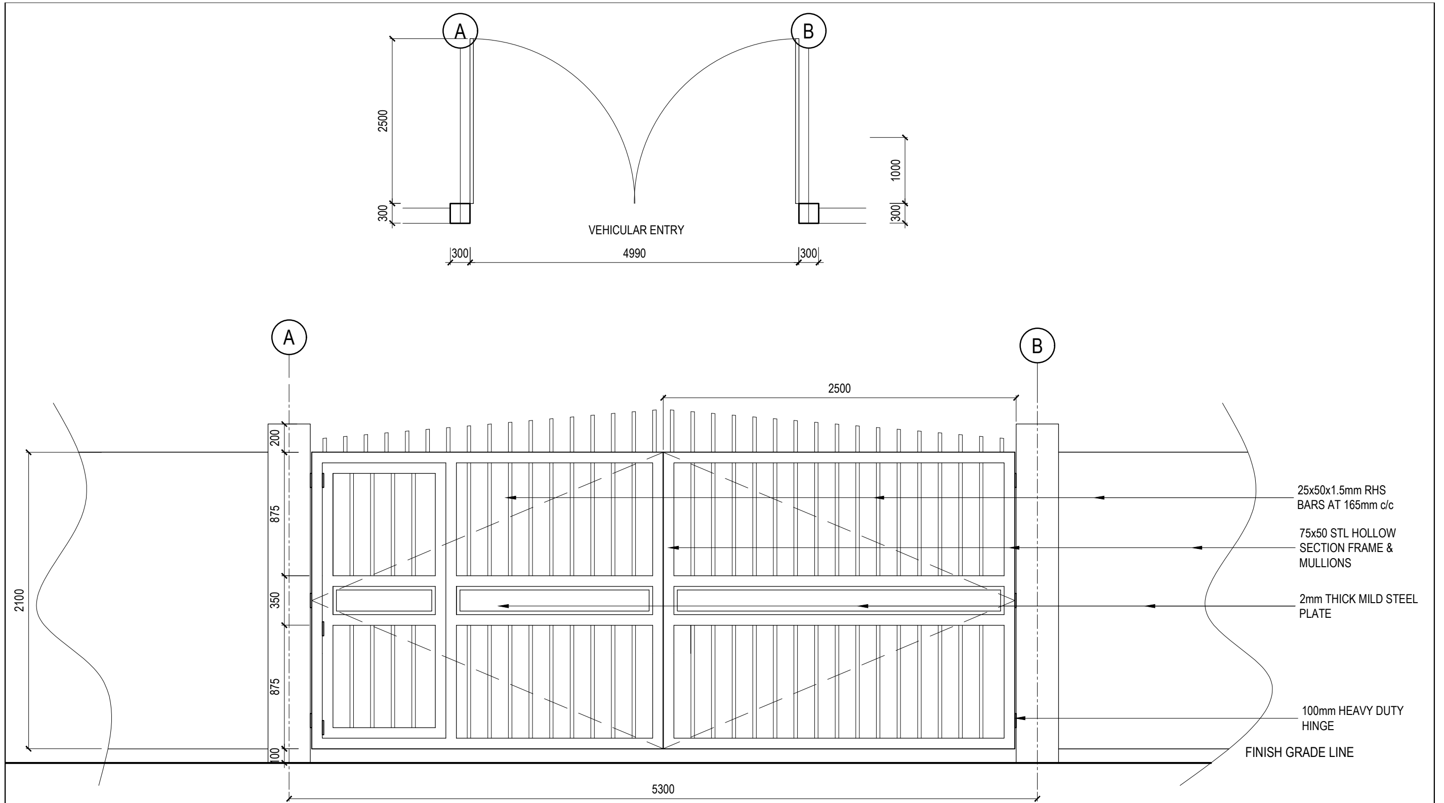
TYPICAL GATE ELEVATION
