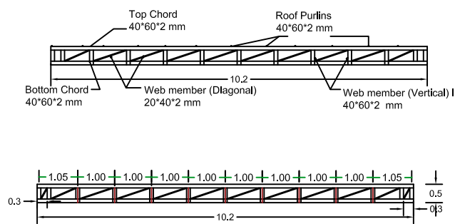
Truss Details
