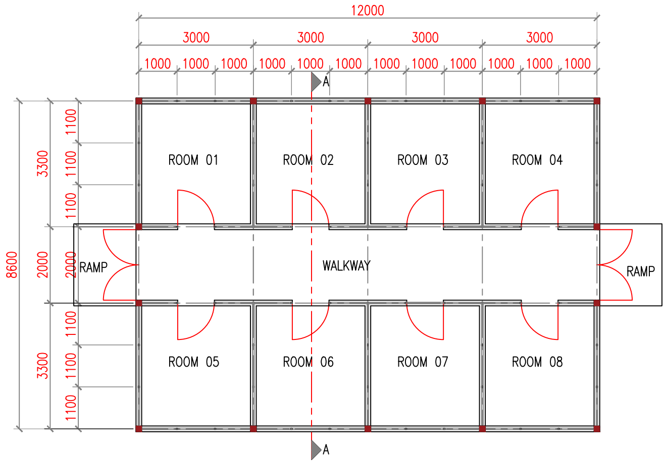
FLOOR PLAN (DELIVERY PEN )
