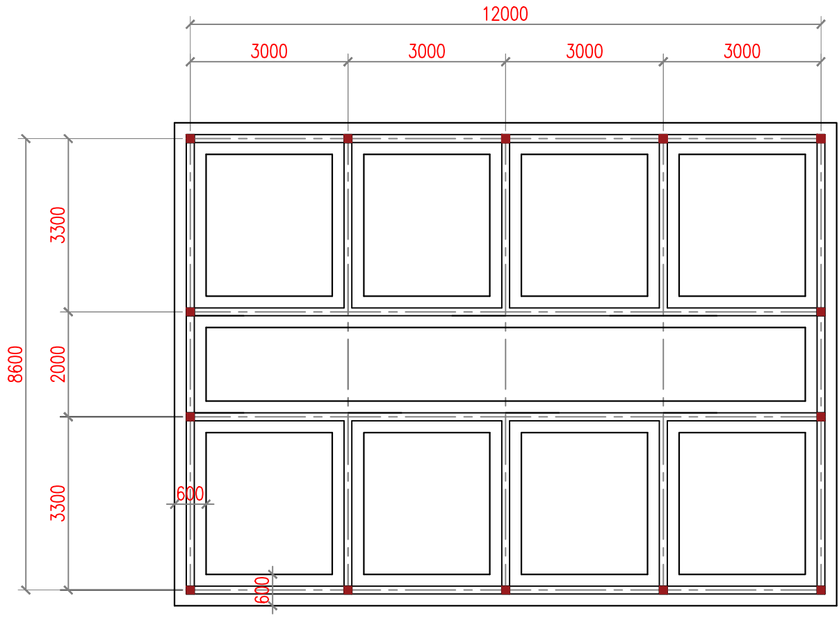
FOUNDATION PLAN (DELIVERY PEN) 1/100
