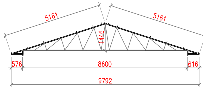
TRUSS TYPE (9NS)
