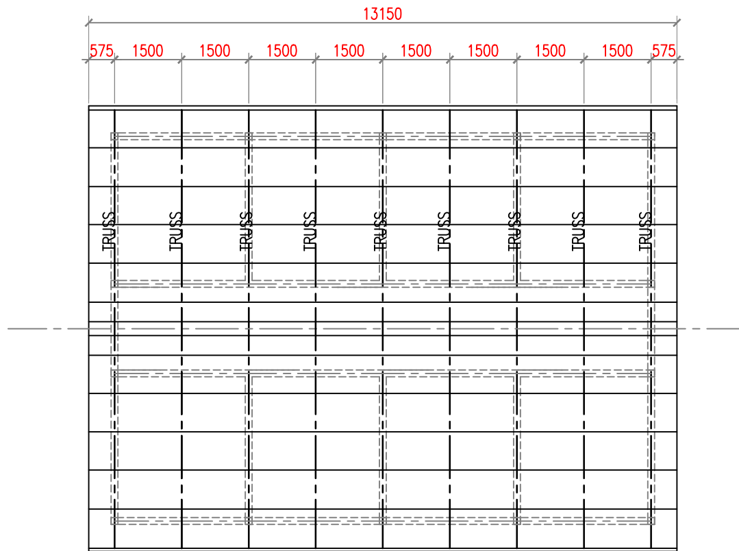
ROOF PLAN (DELIVERY PEN)
