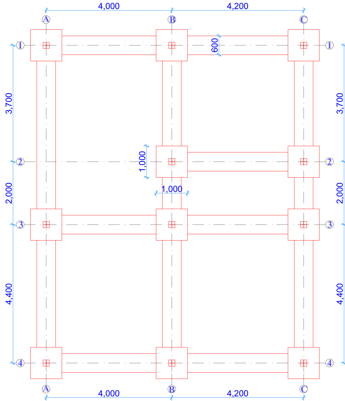
FOUNDATION LAYOUT
