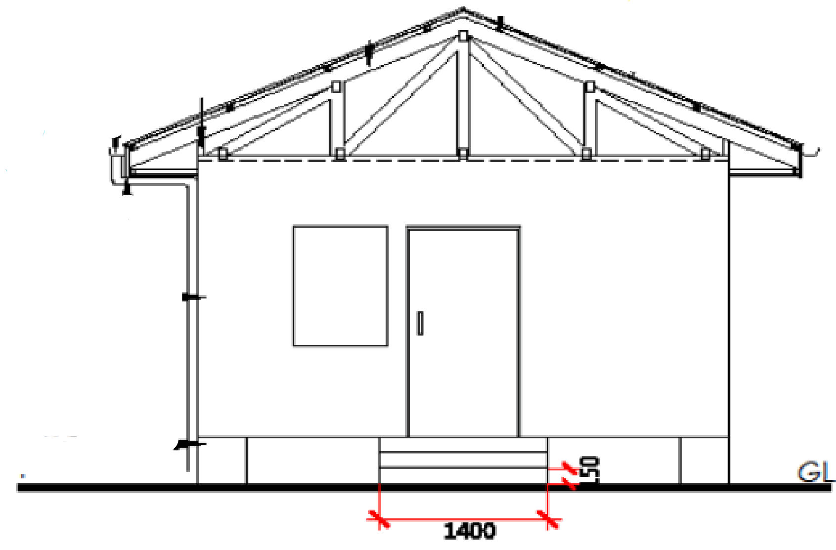
FRONT ELEVATION
