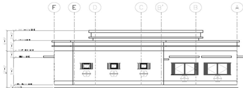
2 REAR SIDE ELEVATION SCALE 1/8" = 1'-0"
