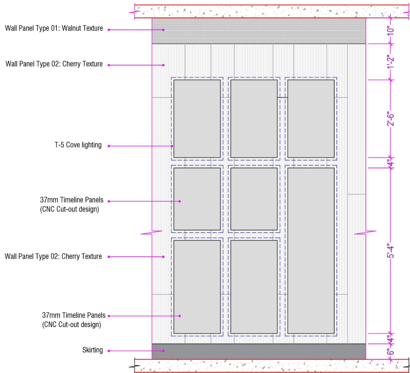
Lobby Timeline Panel Front Elevation
