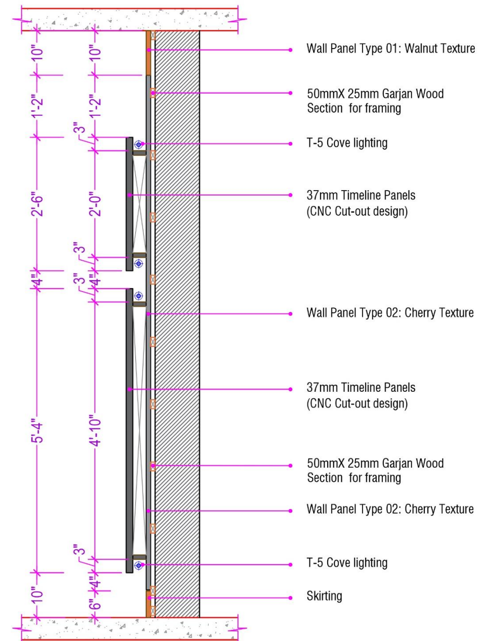
Lobby Timeline Panel Cross Section
