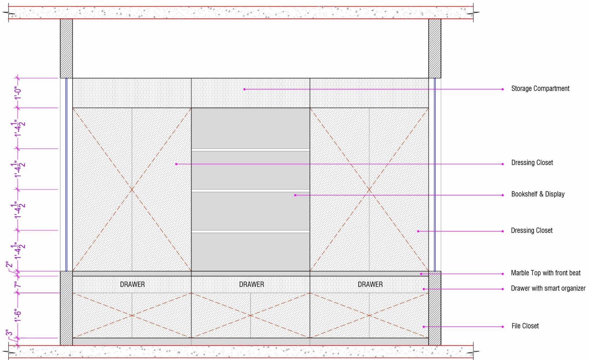
Executive Closet Design Front Elevation
