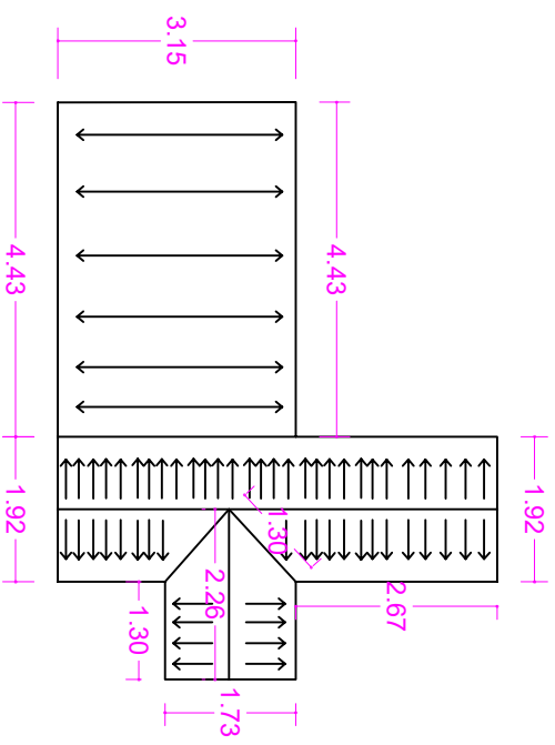
ROOF PLAN
