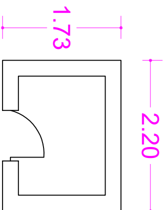
PUMP HOUSE PLAN
