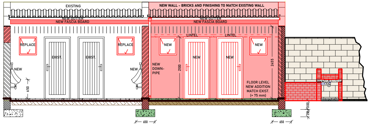
SECTION B-B
