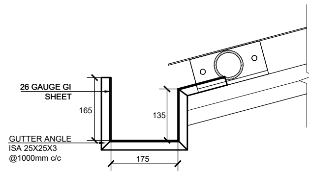
GUTTER DETAILS
