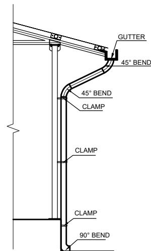
TYPICAL RAIN DROP GUTTER AND PIPE DETAIL
