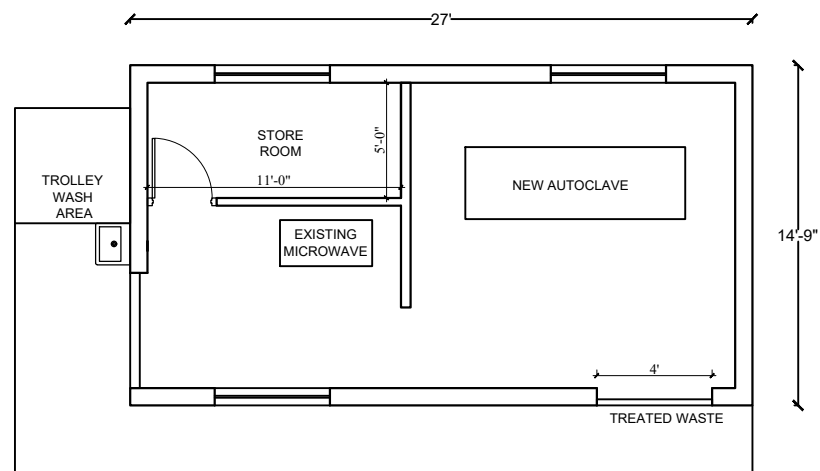
PROPOSED RISK WASTE TREATMENT BLOCK FLOOR PLAN AREA = 398 SQ.FT.
