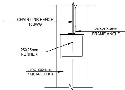
CHAIN LINK DETAIL
