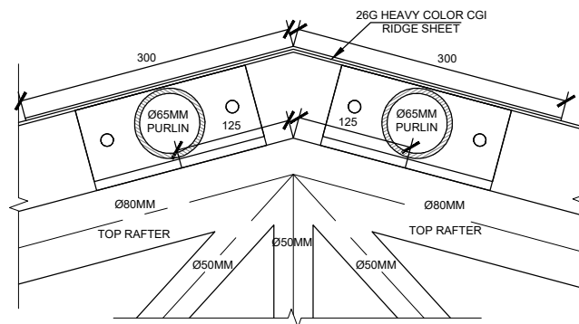
TRUSS DETAIL
