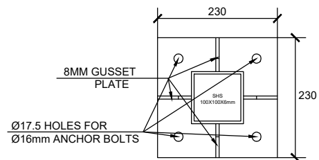
POST DETAILS
