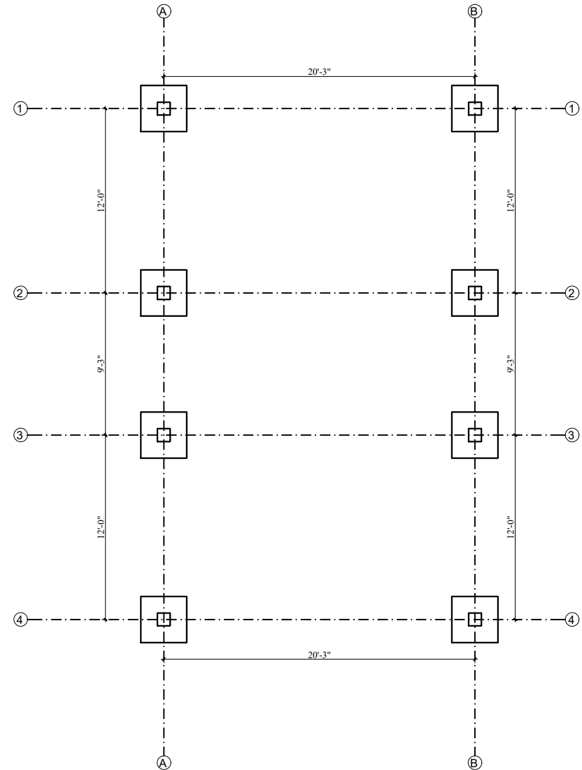
FOOTING PLAN
