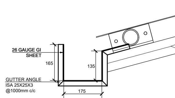
GUTTER DETAILS
