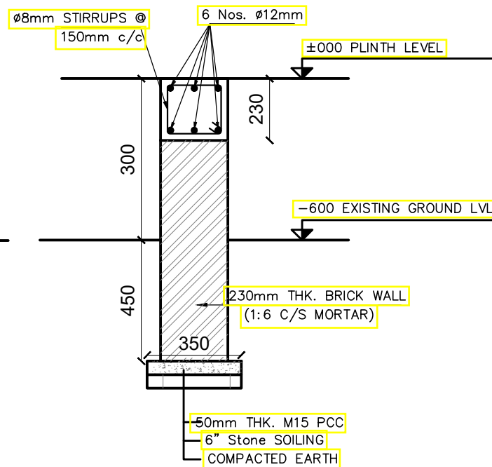
TYPICAL TOE WALL DETAIL (NOT IN SCALE)
