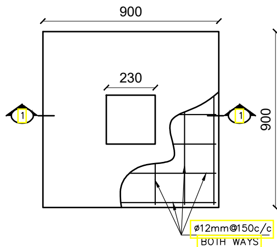
FOOTING (F) PLAN (NOT IN SCALE)
