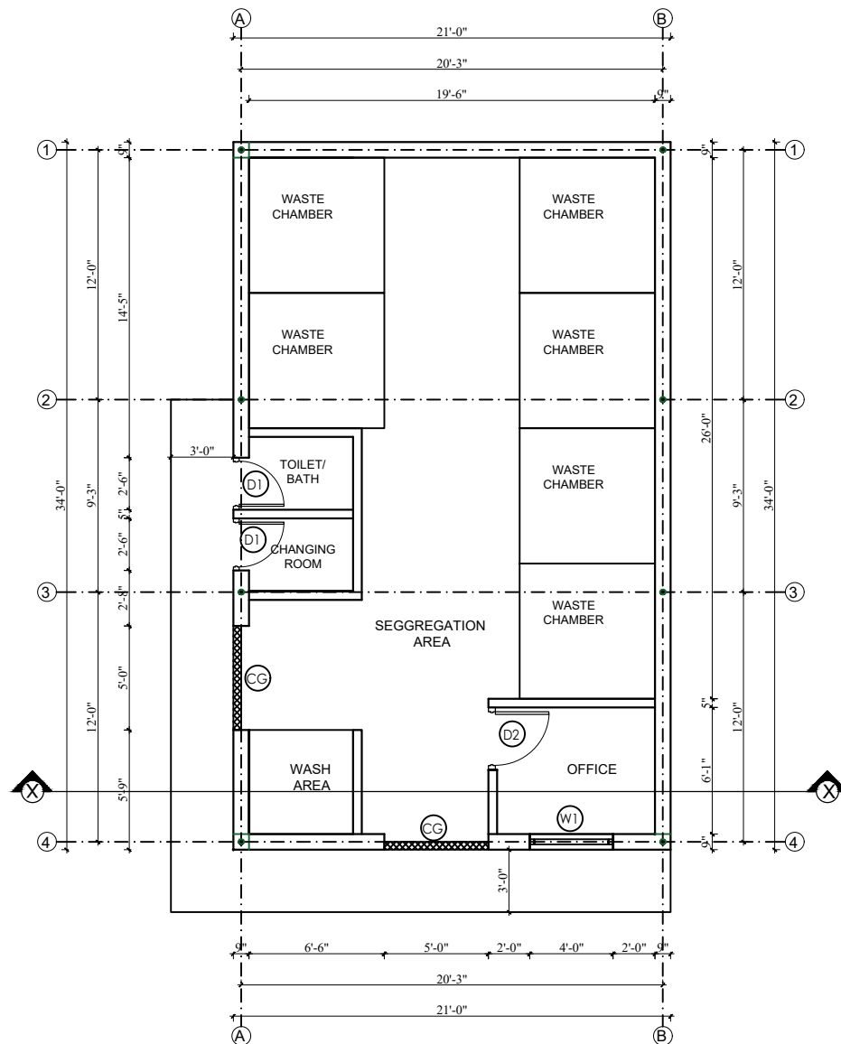
GROUND FLOOR PLAN AREA = 714 SQ.FT. GENERAL WASTE BLOCK - SURKHET
