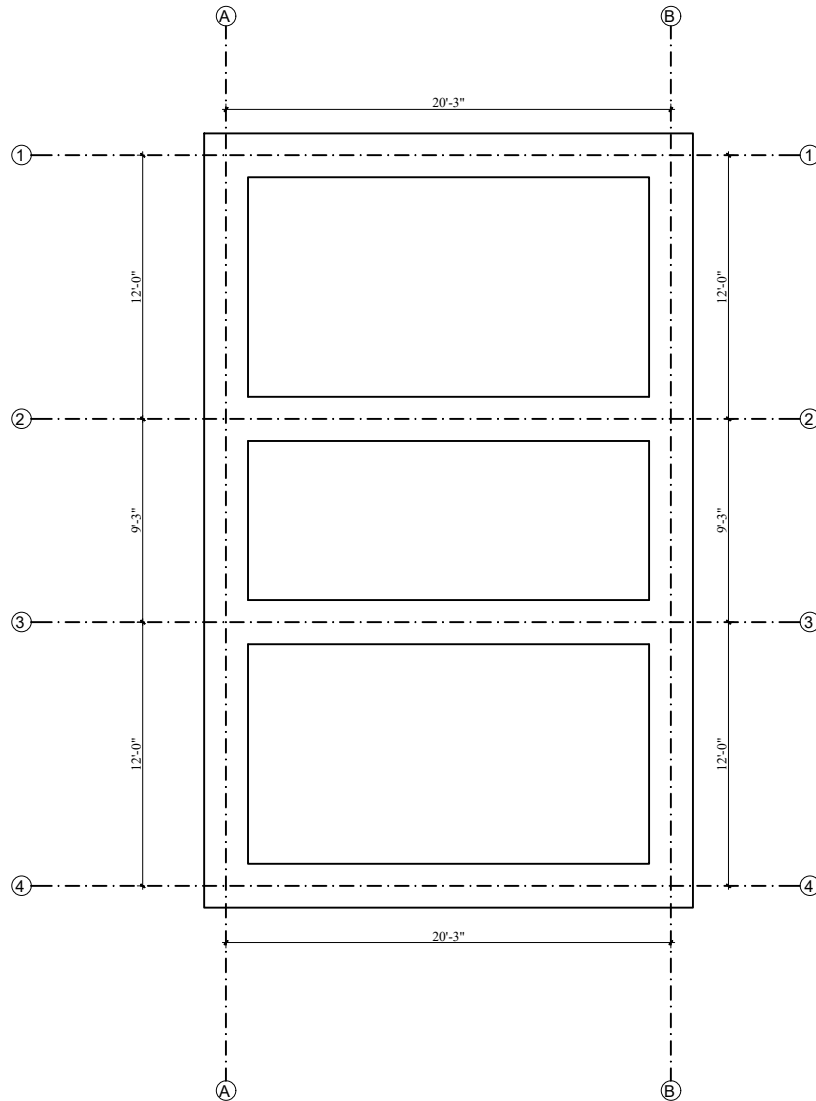
TRENCH PLAN
