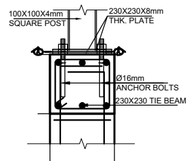
POST/PLINTH BEAM SECTION
