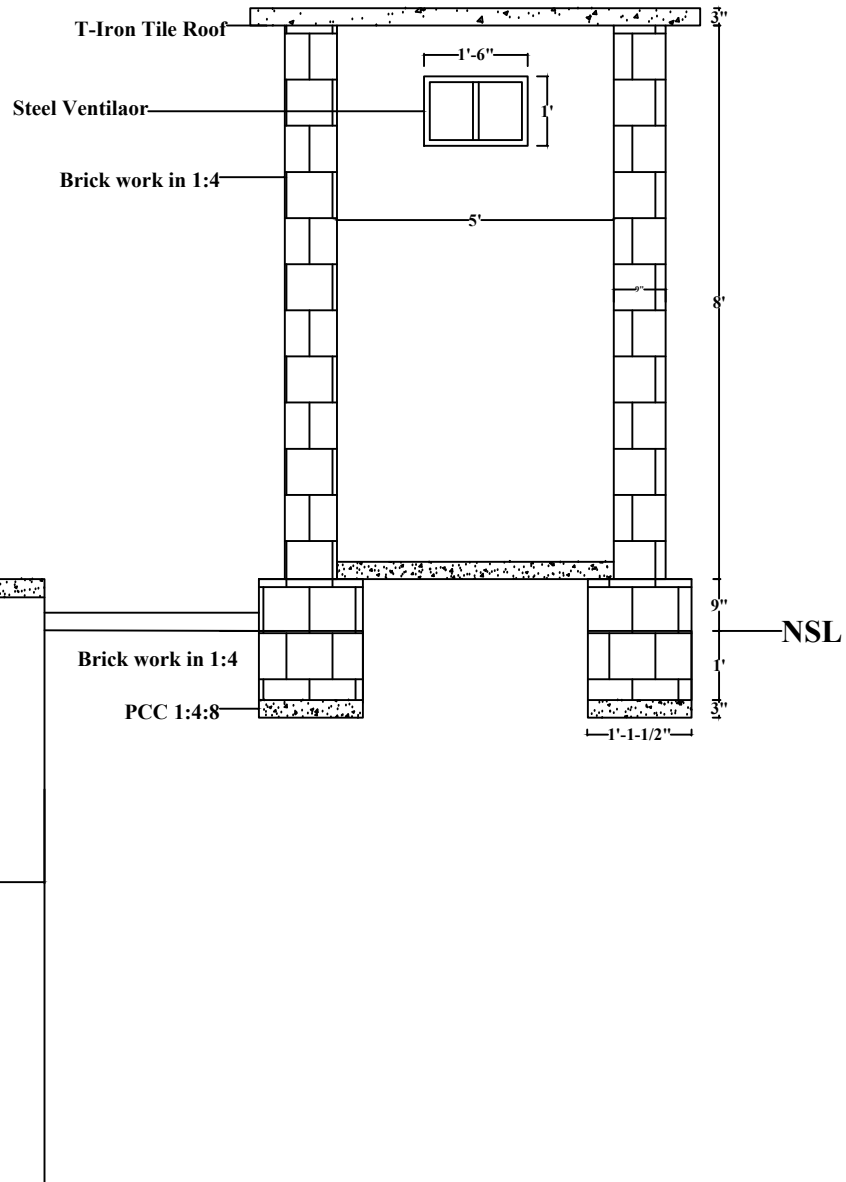
X section & back Elevation of VIP Latrine
