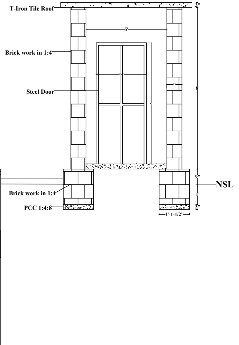
X section of VIP Latrine
